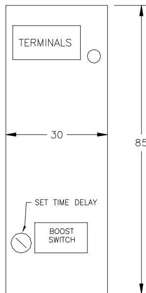
VIEW OF PCB WHEN FITTED
